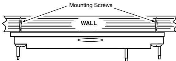
Figure 3: Surface mounting the Sensor
