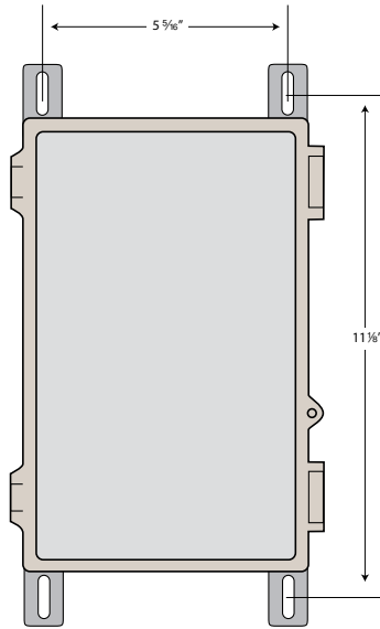
Figure 1: Mounting Dimensions
