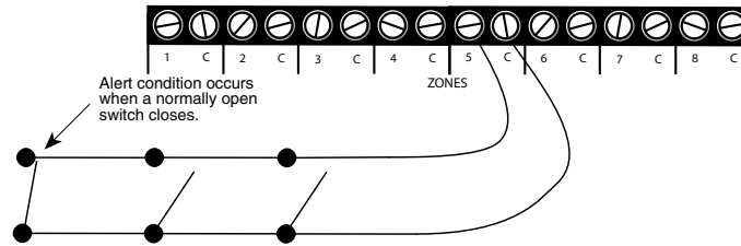
Figure 2-9 Multiple Normally Open Sensors
