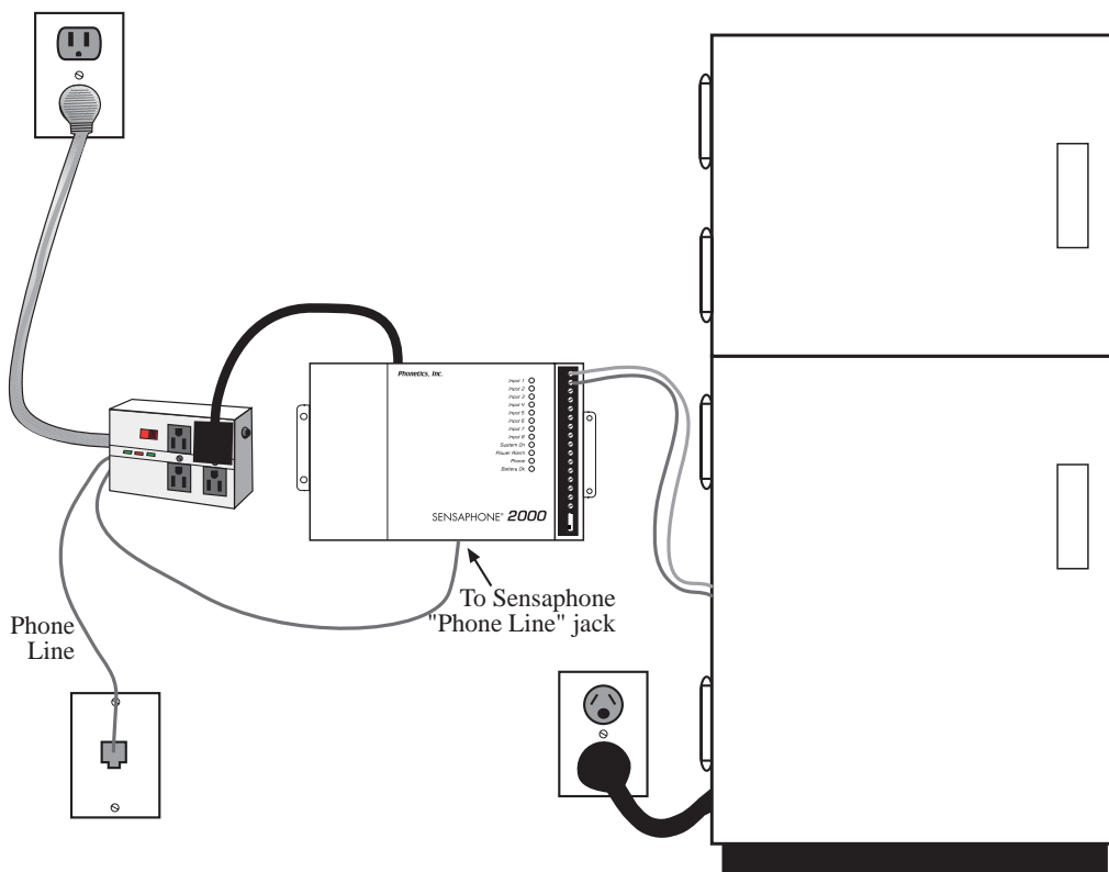
Figure 2: Power Wiring
