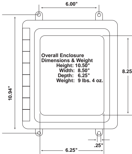
Figure 1: Mounting Express
