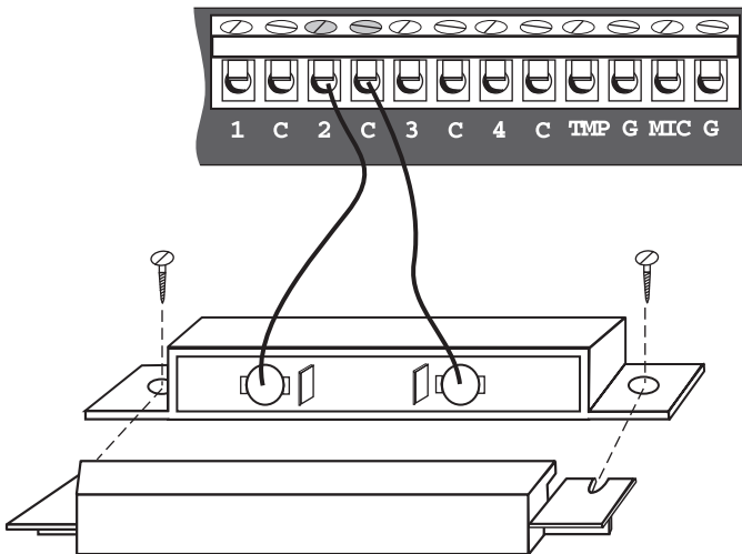
Figure 2: Connecting a sensor to an input terminal
