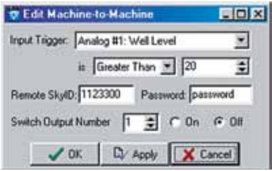
Figure 5: Turn Pump Off if Level is Greater than 20 feet
